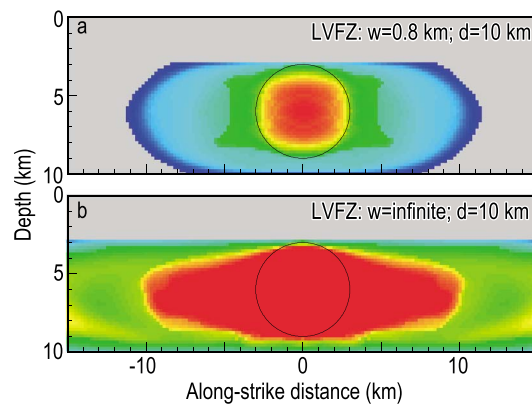
Figure 8. Slip distribution (color) for the models with different LVFZ widths (a) w = 0.8 km, (b) w = \text{infinite} .
