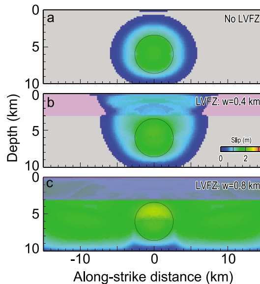
Figure 5. (a–c) Slip distribution (color) for the surface-breaking models, i.e., seismogenic zone range is 0–10 km in depth. The LVFZs are shown as the pink rectangles with \Delta V=40\% . The radius of the nucleation zone is 2.6 km for these cases.
