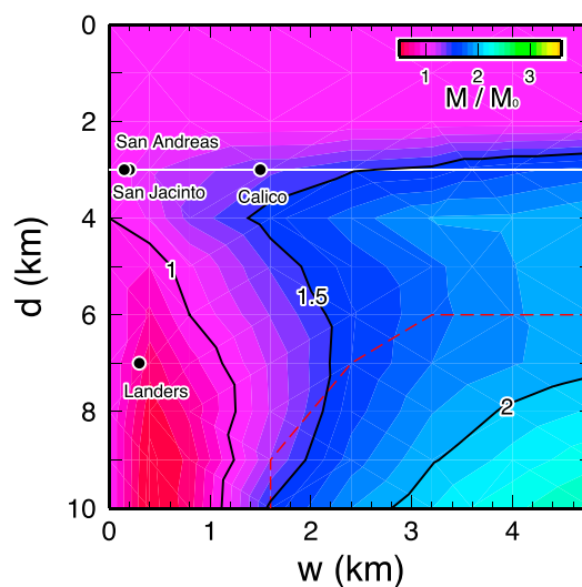
Figure 9. A contour map of the normalized seismic moments (ratios between moments for models with LVFZs and the model without LVFZ, M/M_0 ) on the width and depth extent of the LVFZ. Others are same as in Figure 3a.
